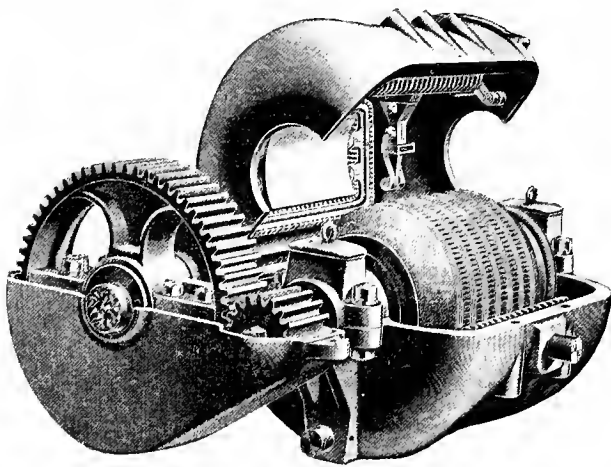
Fig. 5674. MOTOR-CASE AND ATTACHMENT TO AXLE.
